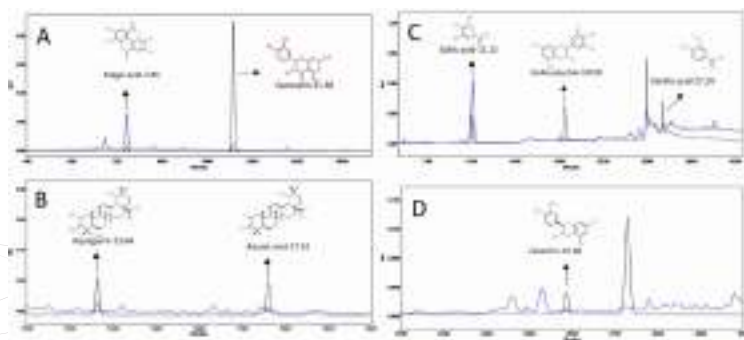
Fig. 1. HPLC-based Phytochemical analysis of the HAV. The different compounds in HAV were A) ellagic acid, and quercetin (at 365 nm wavelength); B) arjungenin, and arjunic acid (at 210 nm wavelength), C) gallic acid, galocatechin, and vanillic acid (at 210 nm wavelength); and D) catechin (at 270 nm wavelength). In the chromatograms, the black line shows the standards for phytochemicals and the blue line indicates the phytochemicals identified in test samples.
