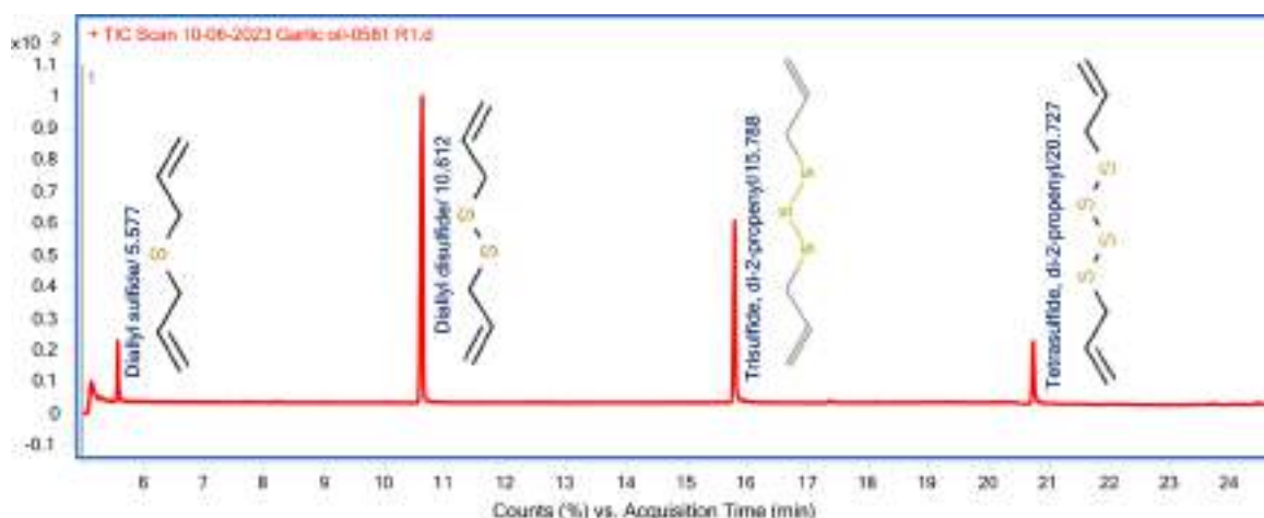
Fig. 2. The GC-MS chromatogram of Cholo garlic pills. The GC-MS chromatogram indicated the presence of diallylsulfide, diallyldisulfide, trisulfide, di-2-propenyl, and tetrasulfide, di-2-propenyl in Cholo garlic pills.
