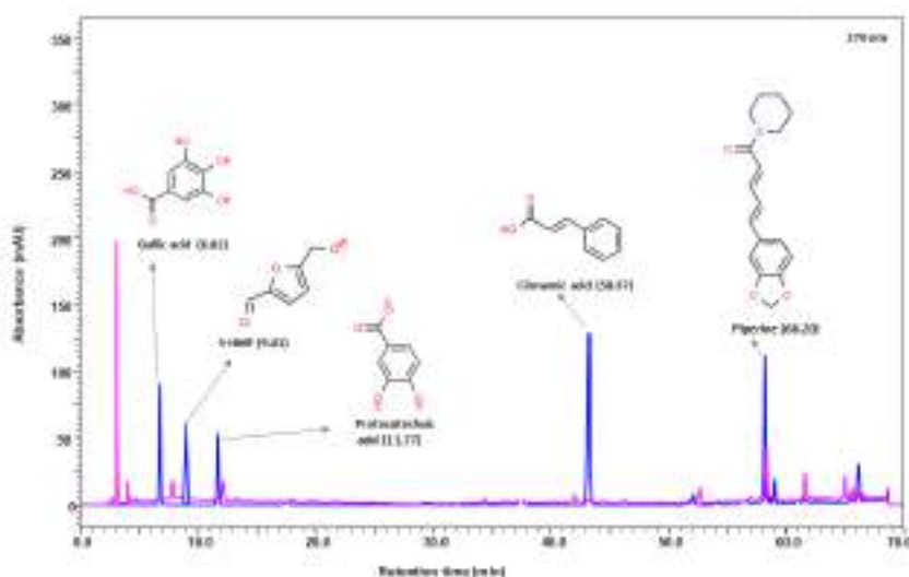
Fig. 1. High Performance Liquid Chromatography (HPLC) with Photo Diode Array Detector (PDA) study confirm that Neurogrit contain gallic acid at 6.82 minute, 5-(hydroxymethyl) furfural (5-HMF) at 9.01 minute, protocatechuic acid at 11.77 minute, cinnamic acid at 58.37 minute, and piperine at 66.20 minute.
