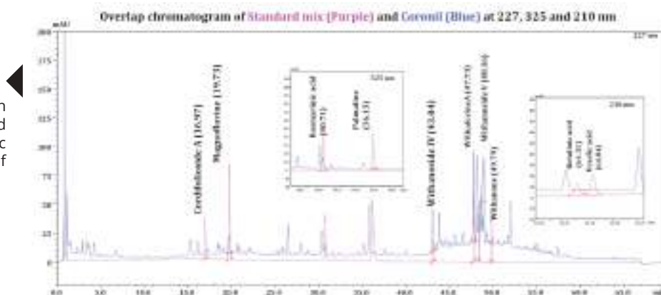
Fig. 3. High Performance Liquid Chromatographic (HPLC) analysis of Coronil tablet.
