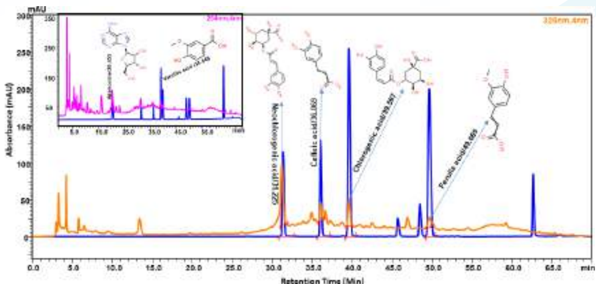
Fig. 1. Ultra High Performance Liquid Chromatography (UHPLC) equipped with Photo Diode Array (PDA) detector analysis of Corighan tablet. In Corighan tablet, the compounds were observed mainly adenosine (20.453 minutes), and vanillic acid (38.848 minutes) at 254 nm wavelength; neochlorogenic acid (31.225 minutes), caffeic acid (36.069 minutes), chlorogenic acid (39.597 minutes), and ferulic acid (49.665 minutes) at 325 nm wavelength. In the chromatograms, the blue line shows the standards and other lines indicate the test sample.
