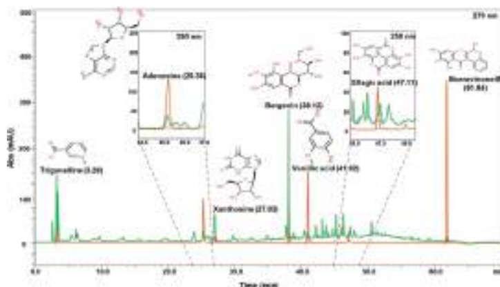
Fig. 2. Quantitative analysis of phytoconstituents of Lithom using Ultra High Performance Liquid Chromatography (UHPLC).
