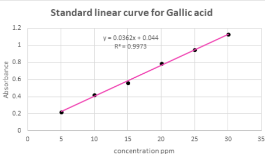
Fig. 1: Calibration curve for total phenolic content using gallic acid as reference standard.
