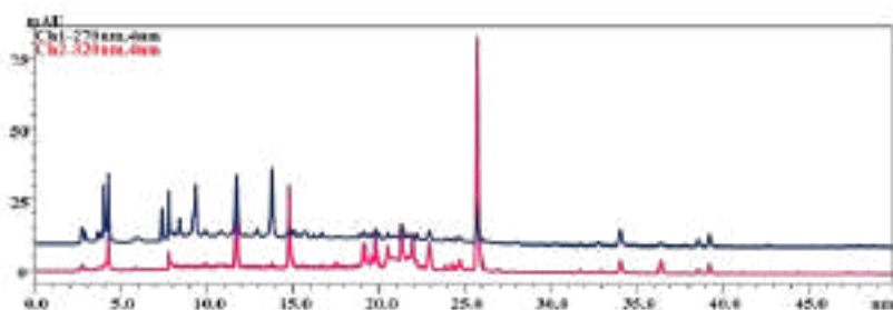
Fig 1: High Performance Liquid Chromatography with PDA (HPLC-PDA) detector at 270 nm and 320 nm wavelength confirms the presence of phytochemicals from Typhogrit. At 270 nm wavelength black chromatogram shows about eight major compounds similarly 320 nm wavelength shows eleven major compounds.
