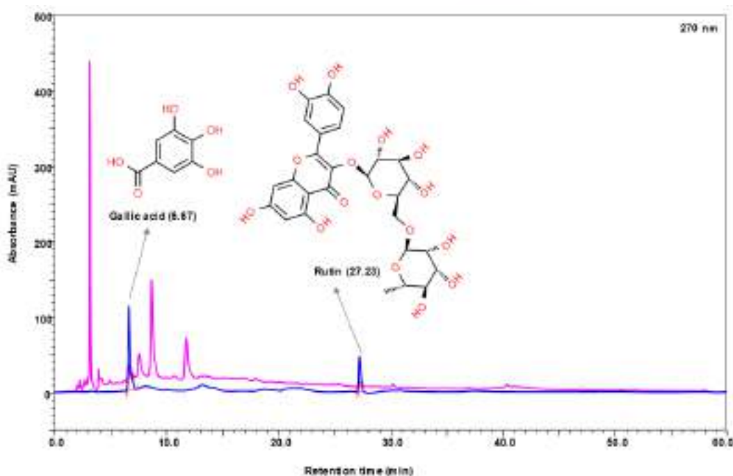
Fig. 1: High Performance Liquid Chromatography (HPLC) chromatogram showing the presence of gallic acid and rutin as major phytoconstituents.
