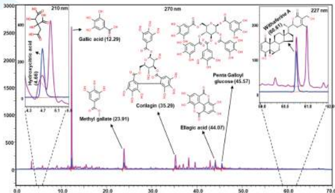
Fig. 2. Phytochemical analysis of Weightgo was performed using Ultra High Performance Liquid Chromatography (UHPLC) equipped with Photo Diode Array Detector (PDA). UHPLC profile recorded at 270 nm wavelength confirms the presence of gallic acid, methyl gallate, corilagin, ellagic acid and penta galloyl glucose. Similarly, at 227 nm wavelength confirms for the presence of withaferin A at 60.61 minutes and at 210 nm wavelength hydroxycitric acid at 4.66 minutes.
