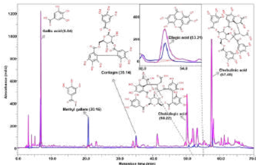
Fig 1: High Performance Liquid Chromatography (HPLC) analysis shows the presence of gallic acid, methyl gallate, corilagin, chebulegic acid, ellagic acid, and chebulinic acid. Blue chromatogram represents the reference standard and pink chromatogram represents Dermagrit Lep, molecular structure and retention times are shown.
