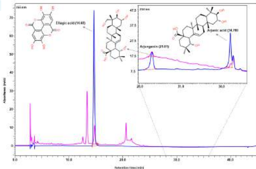
Fig. 1. Ultra High Performance Liquid Chromatography (UHPLC) equipped with Photo Diode Array (PDA) detector analysis of the Cardiogrit tablet. In Cardiogrit tablet, the compounds were observed ellagic acid (14.68 minutes) at 365 nm wavelength; arjungenin (29.01 minutes) and arjunic acid (34.78 minutes) at 210 nm wavelength. In the chromatograms, the blue line shows the standards and pink line indicates the test sample.
