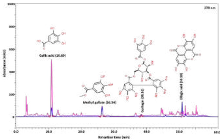
Fig. 1. Analysis of the Nutrela iron complex natural by Ultra High Performance Liquid Chromatography (UHPLC) equipped with Photo Diode Array (PDA) detector. In the Nutrela iron complex natural, the different compounds were observed mainly gallic acid (10.89 minutes), methyl gallate (26.34 minutes), corilagin (38.32 minutes), and ellagic acid (50.90 minutes) at 270 nm wavelength. In the chromatograms, the blue line represents the standards and pink line indicates the test sample.
