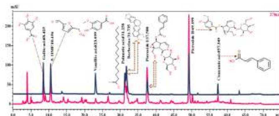
Fig. 1. Ultra High Performance Liquid Chromatography (UHPLC) equipped with Photo Diode Array (PDA) detector analysis of the Livamrit Advance. In Livamrit Advance, the compounds were obtained at 270 nm wavelength mainly: gallic acid (8.425 minutes), 5-hydroxyl methyl furfural (5-HMF) (10.456 minutes), vanillic acid (23.099 minutes), palmaric acid (31.258 minutes), berberine (31.735 minutes), picroside I (37.500 minutes), picroside II (49.199 minutes), and cinamic acid (57.349 minutes). In the chromatograms, the dark blue line shows the standards and red line indicates the test sample.
