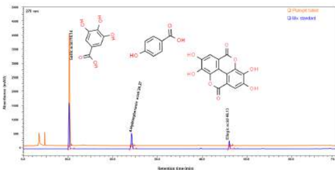
Fig. 1: High Performance Liquid Chromatographic (HPLC) study at 270 nm wavelength confirms the presence of gallic acid, 4-hydroxybenzoic acid, and ellagic acid as major phytoconstituents in Platogrit tablet.
