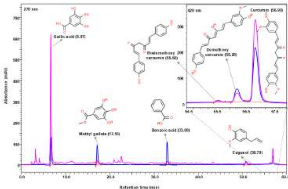
Fig. 1. Ultra High Performance Liquid Chromatography (UHPLC) equipped with Photo Diode Array (PDA) detector analysis of the Eargrit gold tablet. The compounds in Eargrit gold tablet at 270 nm wavelength were mainly gallic acid, methyl gallate, benzoic acid, eugenol and at 420 nm bisdemethoxycurcumin, demethoxycurcumin and curcumin. In the overlay chromatograms, the blue line indicates the standards and pink line represents the test sample.
