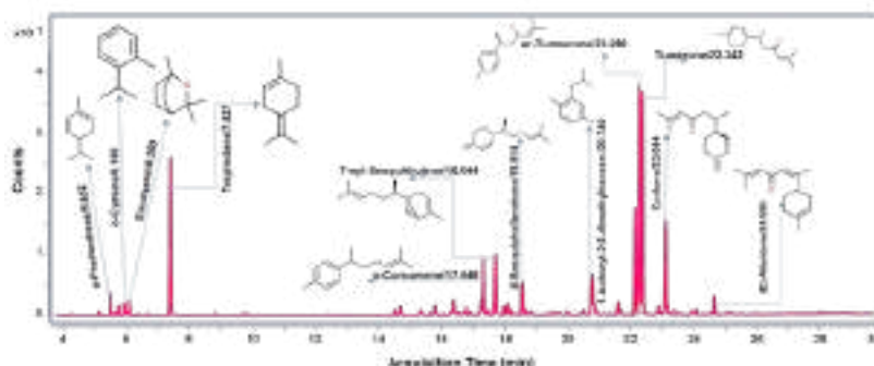
Fig.1.: Gas Chromatography equipped with Quadrupole Mass Spectrometer (GC MS/MS) shown the presence of α-phellandrene, o-cymene, eucalyptol, terpinolene, α-curcumen, 7-epi-sesquithujene, β-sesquiphellandrene, 1-Isobutyl-2,5-dimethylbenzen, curlone, ar-turmerone, tumerone, (E)-Atlantone.
