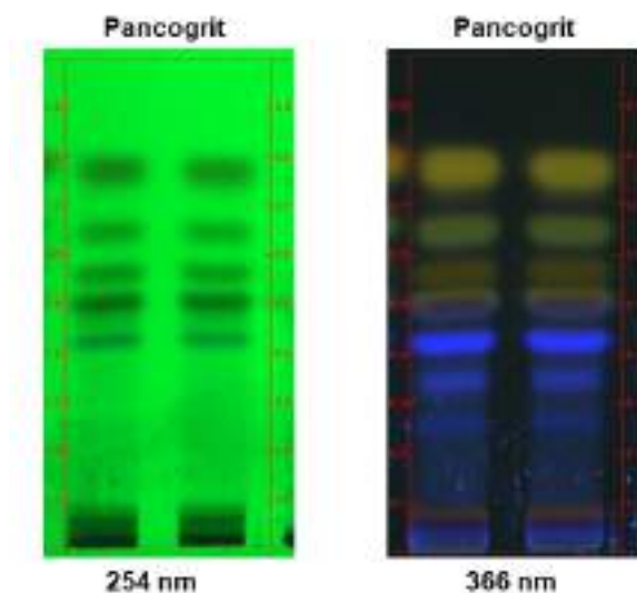
Fig. 1, High Performance Thin Layer chromatography study at 254 nm wavelength confirm the presence of 5 major bands whereas at 366 nm wavelength 6 major bands are observed.
