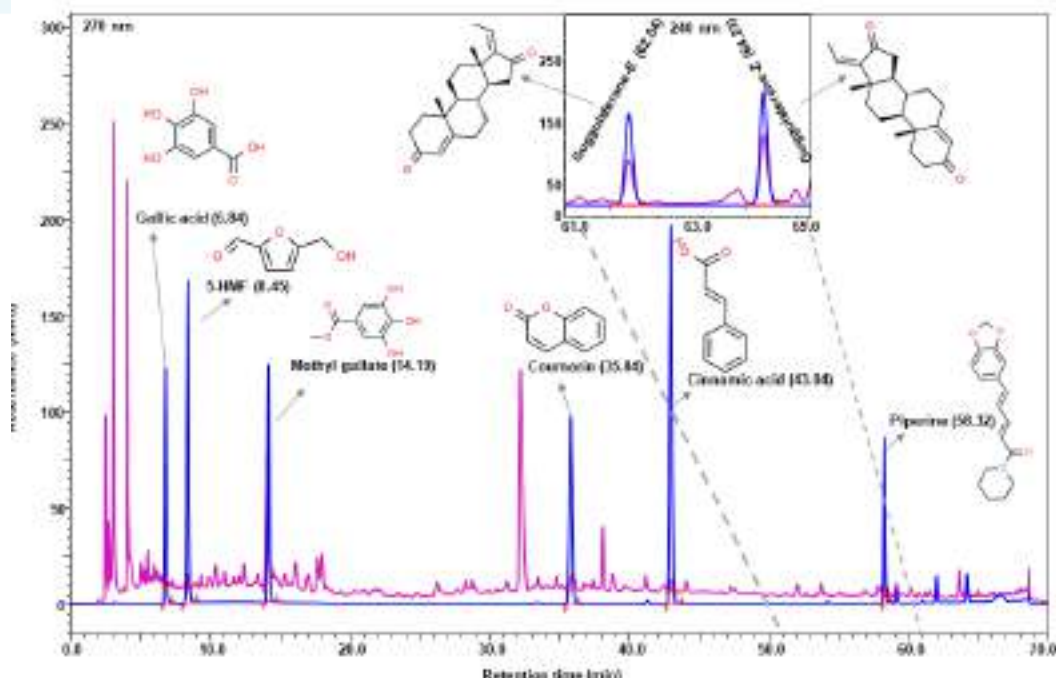
Fig. 1. Analysis of Prostogrit tablet by Ultra High Performance Liquid Chromatography (UHPLC) equipped with Photo Diode Array (PDA) detector. In Prostogrit tablet, the different compounds were observed mainly gallic acid, 5-hydroxyl methyl furfural (5-HMF), methyl gallate, coumarin, cinnamic acid, and piperine at 270 nm wavelength; guggulsterone-E and Z at 240 nm wavelength. In the chromatograms, the blue line represents standards and the pink line represents the test sample.
