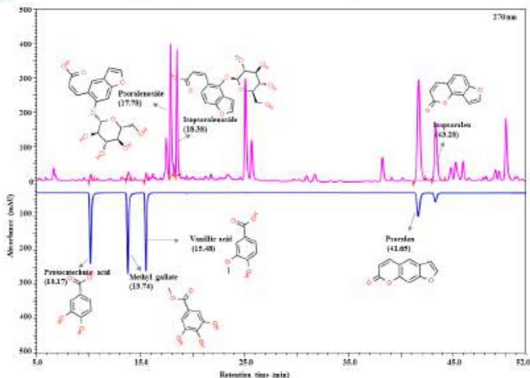
Fig. 1. Ultra High Performance Liquid Chromatography (UHPLC) equipped with Photo Diode Array (PDA) detector analysis of the Melanogrit Gold. In Melanogrit Gold, different compounds were observed at 270 nm wavelength mainly protocatechuic acid, methyl gallate, vanillic acid, psoralenoside, isopsoralenoside, psoralen, and isopsoralen. In the chromatograms, the pink line represents the test sample and inverted blue line represents standards, as shown in Fig. 1.
