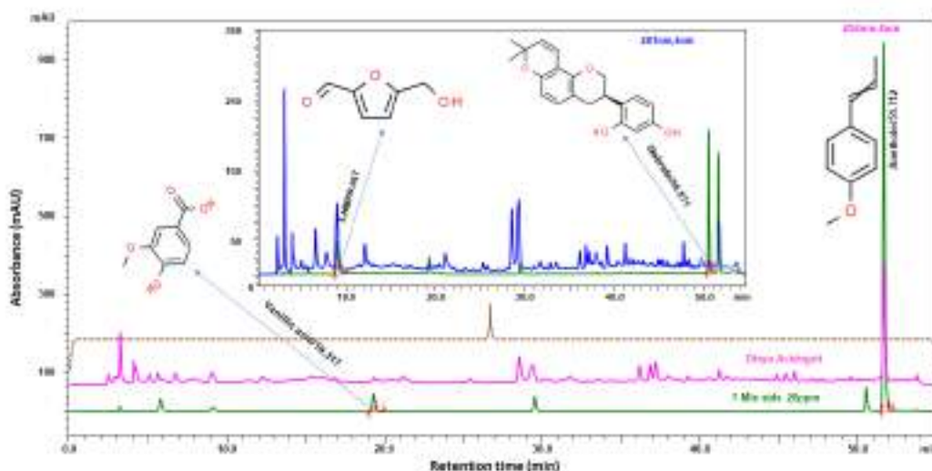
Fig.1. Ultra High Performance Liquid Chromatography (UHPLC) equipped with Photo Diode Array (PDA) detector analysis of the Acidogrit tablet. In Acidogrit tablet analysis, the various compounds were observed mainly vanillic acid (19.317 minutes), and anethole (51.712 minutes) at 254 nm wavelength; 5-hydroxyl methyl furfural (5-HMF) (9.067 minutes), and glabridin (50.571 minutes) at 281 nm wavelength. In the chromatograms, the green line shows the mix standards and pink line indicates the test sample.
