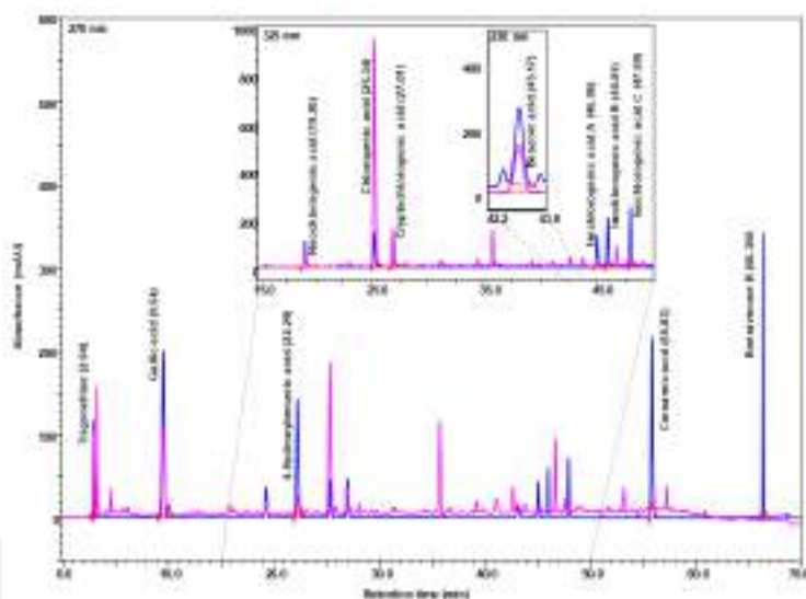
Fig. 1. Analysis of KshyaNIL by Ultra High Performance Liquid Chromatography (UHPLC) equipped with Photo Diode Array (PDA) detector. In KshyaNIL, the different compounds were obtained at 270 nm wavelength mainly trigonelline (2.94 minutes), gallic acid (9.54 minutes), 4-hydroxybenzoic acid (22.29 minutes), cinnamic acid (55.83 minutes), and boeravinone B (66.34 minutes); neochlorogenic acid (19.26 minutes), chlorogenic acid (25.34 minutes), cryptochlorogenic acid (27.01 minutes), isochlorogenic acid A (45.06 minutes), isochlorogenic acid B (46.01 minutes), isochlorogenic acid C (47.99 minutes) at 325 nm wavelength; benzoic acid (43.17 minutes) at 230 nm wavelength. In the chromatograms, the blue line indicates the standards and pink line indicates the test sample.
