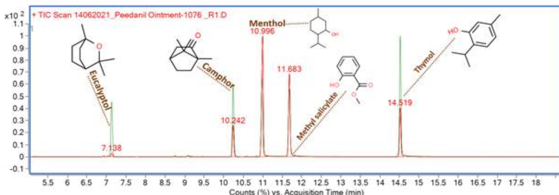
Fig. 1. The Gas chromatography-mass spectrometry (GC-MS) chromatogram of Peedanil Ointment. The GC-MS chromatogram showed the presence of eucalyptol, camphor, menthol, methyl salicylate, and thymol in Peedanil Ointment.
