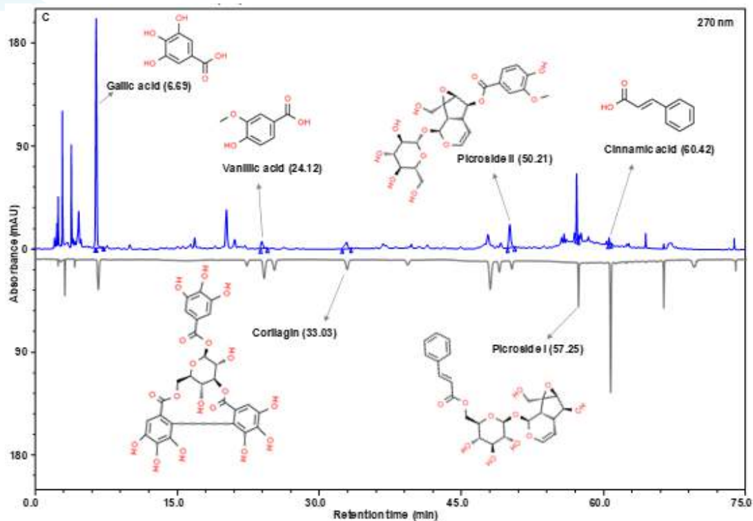
Fig. 1. Analysis of the Madhunashni Vati by Ultra High Performance Liquid Chromatography (UHPLC) equipped with Photo Diode Array (PDA) detector. In Madhunashni Vati, the compounds were obtained at 270 nm wavelength mainly gallic acid (6.69 minutes), vanillic acid (24.12 minutes), corilagin (33.03 minutes), picroside II (50.21 minutes), picroside I (57.25 minutes), and cinnamic acid (60.42 minutes); at 325 nm wavelength caffeic acid (22.29 minutes), chlorogenic acid (25.18 minutes), and rutin (48.89 minutes); at 365 nm wavelength ellagic acid (47.36 minutes). In the chromatograms, the black line shows the standards and blue line indicates the test sample.
