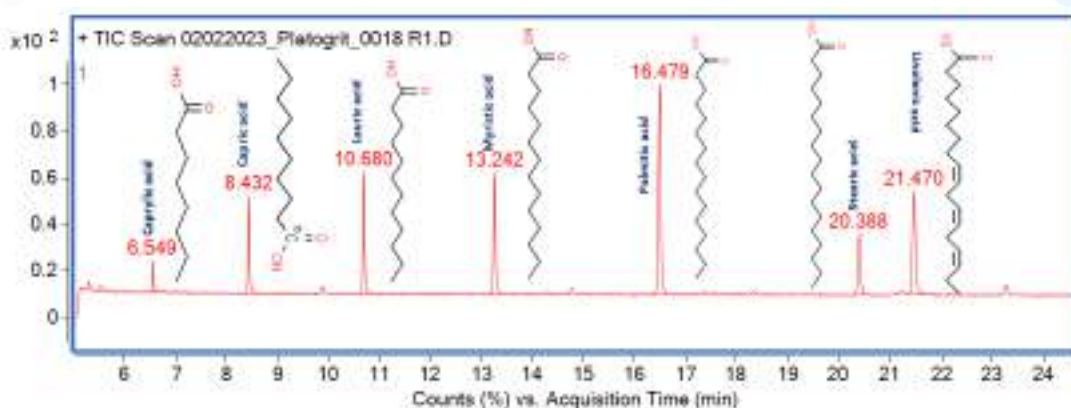
Fig. 2. The GC-MS chromatogram of Platogrit milk granules. The chromatogram showed the presence of different compounds caprylic acid, capric acid, lauric acid, myristic acid, palmitic acid, stearic acid, and linolenic acid in Platogrit milk granules.
