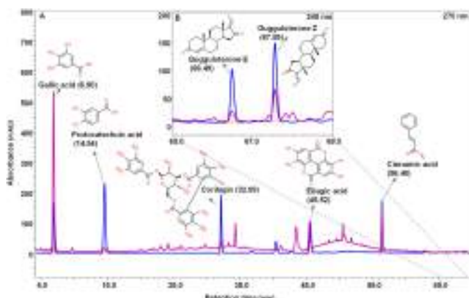
Fig. 2. Phytochemical analysis of Lipidom by UHPLC using PDA detector. Overlap chromatogram of standard mix (blue line) and Lipidom (pink line) confirms the presence of gallic acid, protocatechuic acid, corilagin, ellagic acid, cinnamic acid at 270 nm wavelength and Guggulsterone E and Guggulsterone Z at 240 nm
