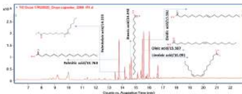
Fig.2.: Fatty acid composition present in Divya capsule are analyzed by Gas Chromatography with Quadrupole Mass Spectrometer (GC MS/MS) are palmitic acid, palmitoleic acid, stearic acid, elaidic acid, oleic acid, linoleic acid. The chemical structure of the representative compounds are provided with the chromatogram.
