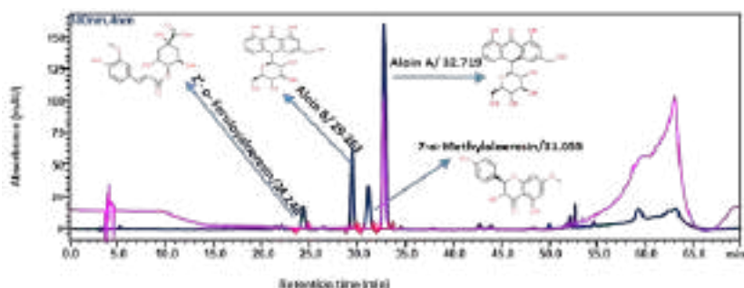
Fig 1: High Performance Liquid Chromatography (HPLC) analysis at 300 nm wavelength of Aloe Kanti Gel shows the presence of 2''-O-feruloylolesin, aloin B, aloin A, and 7-O-methylaloesin which are main constituents of Aloe vera.
