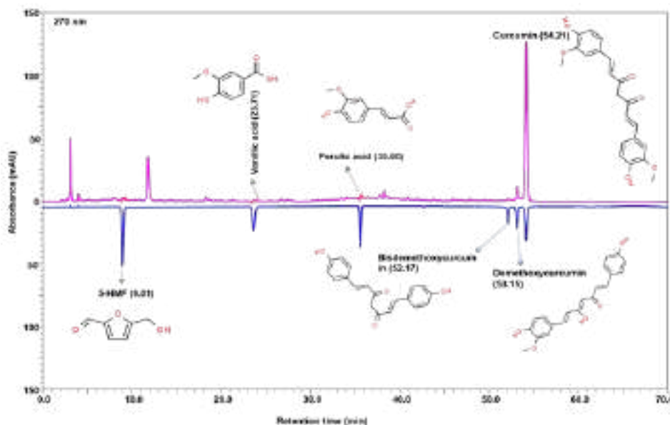
Fig. 1. Ultra High Performance Liquid Chromatography (UHPLC) equipped with Photo Diode Array (PDA) detector analysis of Cystogrit tablet. In Cystogrit tablet, the compounds were observed mainly 5-HMF (9.01 minutes), vanillic acid (23.71 minutes), ferulic acid (35.60 minutes), bisdemethoxycurcumin (52.17 minutes), desmethoxycurcumin (53.15 minutes), and curcumin (54.21 minutes) at 270 nm wavelength. In the chromatograms, the blue line shows the standards and pink line indicates the test sample.
