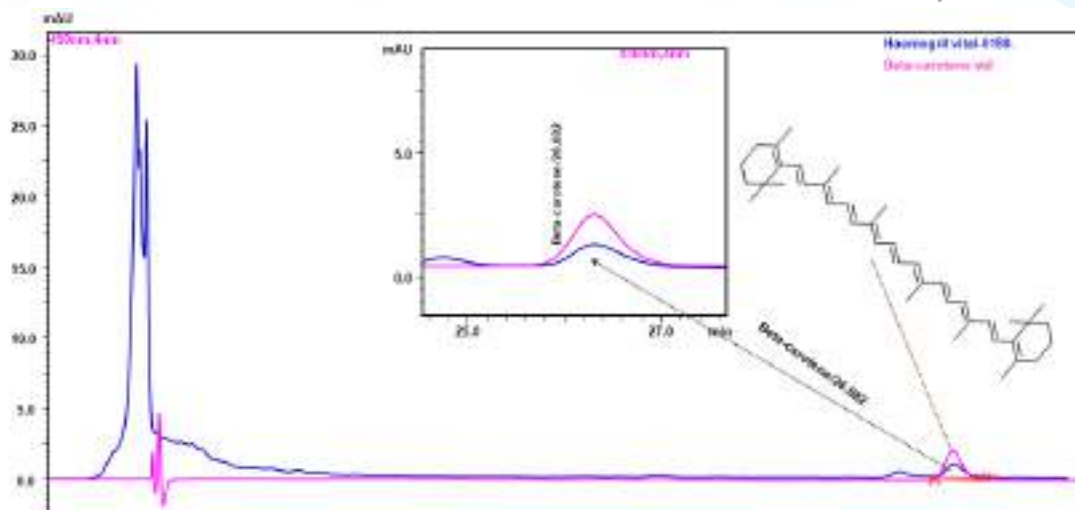
Fig. 3. Ultra High Performance Liquid Chromatography (UHPLC) equipped with Photo Diode Array (PDA) detector analysis of Haemogrit Vital tablet. In Haemogrit Vital tablet, the compound was found mainly \beta -carotene (26.682 minutes) at 450 nm wavelength. In the chromatograms, the red line shows the standard and blue line indicates the test sample.
