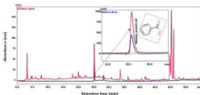
Fig. 1. Ultra High Performance Liquid Chromatography (UHPLC) equipped with Photo Diode Array (PDA) detector analysis of Santati sudha. In Santati sudha, the main compound was found benzoic acid at 230 nm wavelength. In the chromatograms, the dark blue line shows the standard and pink line indicates the test sample.
