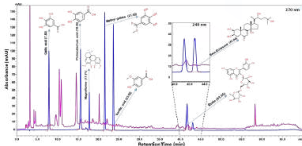
Fig. 1: Ultra Performance Liquid Chromatography (UHPLC) combine with Photo Diode Array Detector (PDA) confirm the presence of gallic acid at 7.85 minutes, protocatechuic acid at 15.56 minutes, magnoflorine 17.17 minutes, methyl gallate at 21.52 minutes, vanillic acid 23.62 minutes, and rutin at 41.65 minutes on analyzing at 270 nm wavelength. Similarly, at 240 nm wavelength beta ecdysone was observed at 43.04 minutes.
