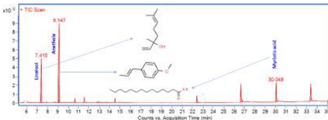
Fig 1: Gas Chromatography with mass detector (GC MS/MS) profile of Shila Tulsi Drop. Molecular structure with a retention time of major constituents, linalool, anethole, and myristic acid shown.
