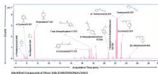
Fig. 1 Gas chromatography equipped with mass detector (GC MS/MS) confirm the presence of \alpha -phellandrene (retention time: 5.648 minute), o-Cymene (retention time: 6.041 minute), Eucalyptol (retention time: 6.209 minute), Terpinolene (retention time: 7.441 minute), \alpha -Curcumene (retention time: 17.312 minute), 7-epi-Sesquithujene (retention time: 17.673 minute), \beta -Sesquiphellandrene (retention time: 18.544 minute), 1-Isobutyl-2,5-dimethylbenzen (retention time: 20.765 minute), ar-Turmerone (retention time: 22.274 minute), Tumerone (retention time: 22.357 minute), Curlone (retention time: 23.078 minute), (E)-Atlantone (retention time: 24.624 minute).
