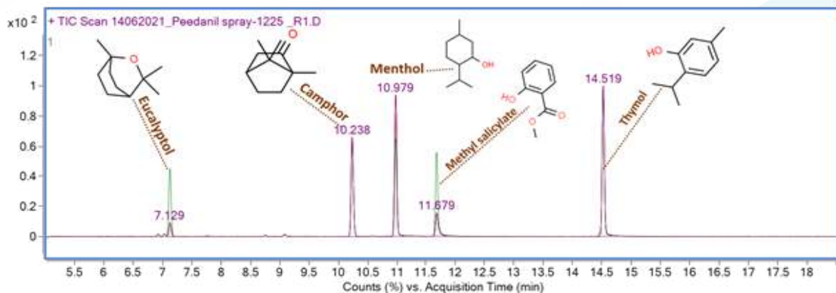
Fig. 1. The Gas chromatography-mass spectrometry (GC-MS) chromatogram of Peedanil Spray and Roll-On. The GC-MS chromatogram indicated the existence of different compounds eucalyptol, camphor, menthol, methyl salicylate, and thymol in Peedanil Spray and Roll-On.
