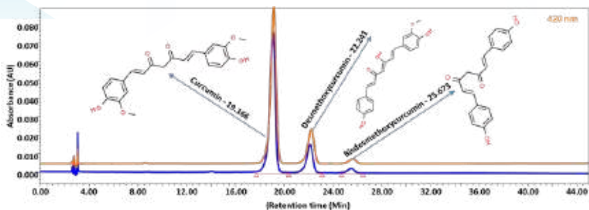
Fig 1: High Performance Liquid Chromatography (HPLC) at 420 nm of wavelength confirms the presence of curcuminoids (curcumin, desmethoxycurcumin and bisdesmethoxycurcumin).
