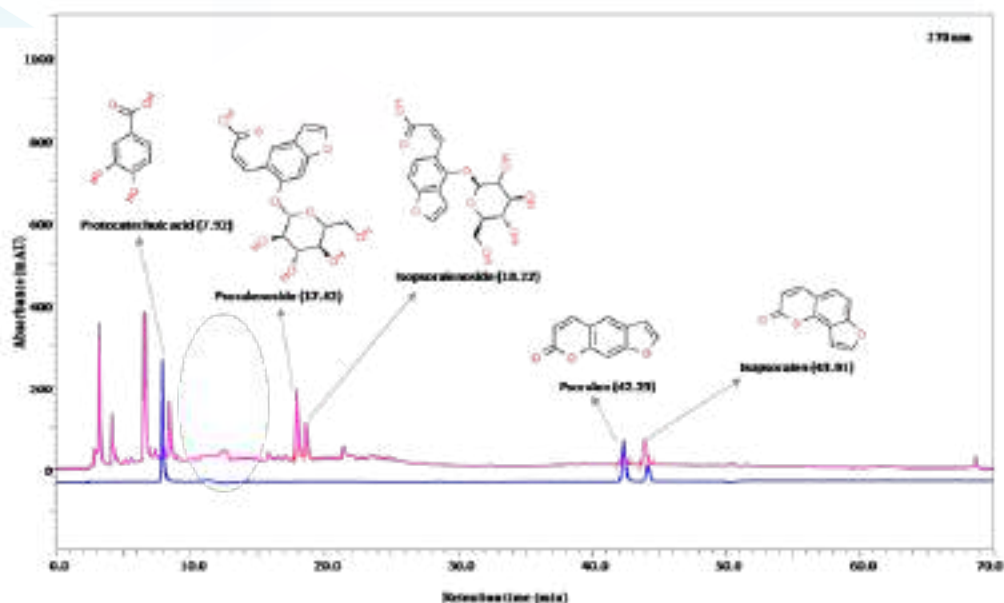
Fig. 1. Ultra High Performance Liquid Chromatography (UHPLC) equipped with Photo Diode Array (PDA) detector analysis of the Melanogrit Lep. In Melanogrit Lep, the compounds were obtained at 270 nm wavelength: A) Protocatechuic acid, B) Psoralenoside, C) Isopsoralenoside, D) Psoralen , E) Isopsoralen. In the chromatograms, the blue line represents standards and the pink line represents the test sample.
