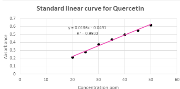
Fig. 2: Calibration curve for total flavonoid content using quercetin as reference standard.
