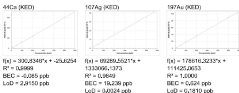
Fig. 1: Inductively Coupled Plasma Mass Spectrometry (ICP-MS) analysis calibration curve at different concentration. R^2 value greater than 0.98 confirms the accuracy and presence of calcium (Ca), silver (Ag), and Gold (Au).
