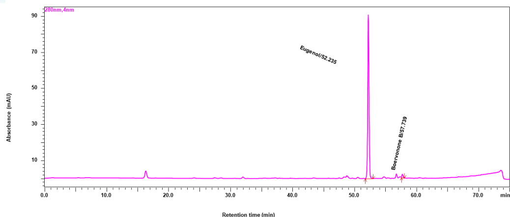
Fig. 1. Analysis of the Eyegrit eye drops by Ultra High Performance Liquid Chromatography (UHPLC) equipped with Photo Diode Array (PDA) detector. The two main compounds were obtained Eugenol (52.235 minutes) and Boervonone (57.739 minutes) at 280 nm wavelength. In the chromatograms, the blue line indicates the standards and pink line shows the test sample.
