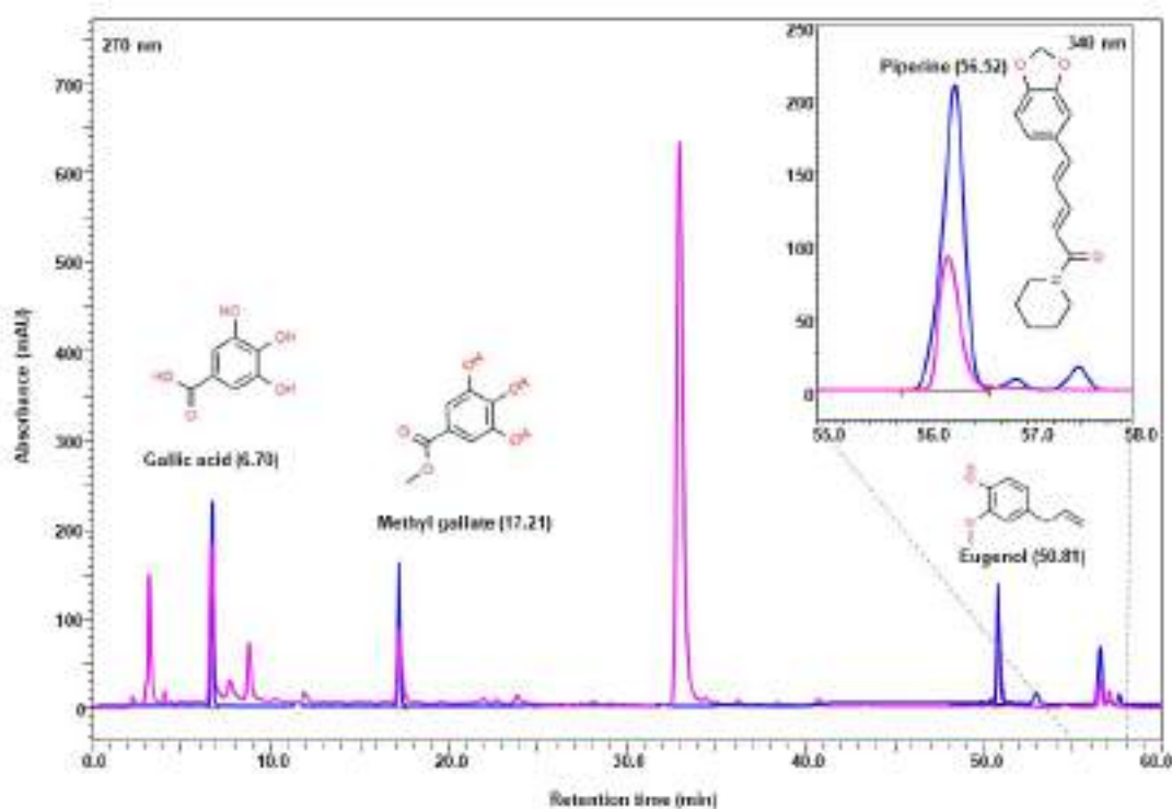
Fig 1: High Performance Liquid Chromatography (HPLC) method shows the presence of gallic acid, methyl gallate, eugenol at 270 nm wavelength and piperine at 340 nm wavelength. Blue chromatogram represent reference standard and pink represent Kanthamrit.
