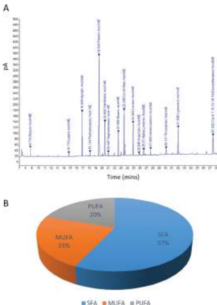
FIG. 1 Gas chromatography–flame ionized detector (GC–FID) chromatogram of Sea Buckthorn oil (SBKT). (A) The fatty acid composition of the SBKT was calculated by using the GC–FID methodology. Individual fatty acids were identified and quantified using fatty acid methyl ester methodology. Chromatography analysis identified 16 major fatty acids. (B) Pie-diagram represents the percentage of 3 categories of fatty acids identified in the SBKT—saturated fatty acids (SFA), monounsaturated fatty acids (MUFA), and polyunsaturated fatty acids (PUFA).
