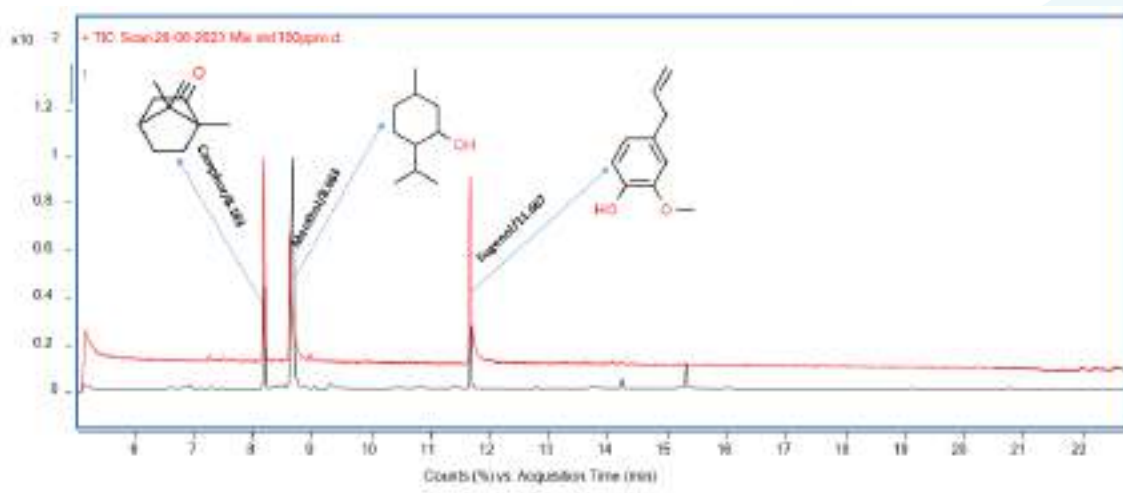
Fig 2: Gas Chromatography with mass detector (GC MS/MS) confirms the presence of camphor, menthol and eugenol in kanthamrit tablet.
