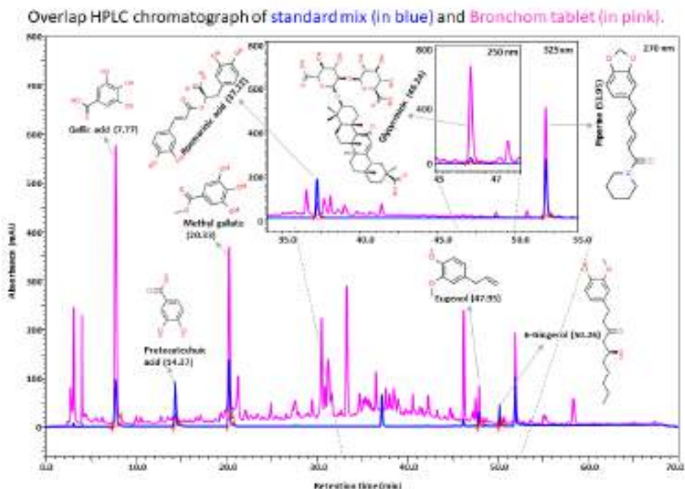
Fig.1: Ultra High Performance Liquid Chromatograph (UHPLC) study of Bronchom confirms the presence of gallic acid, protocatechuic acid, methyl gallate, rosmarinic acid, glycyrrhizin, eugenol, piperine, and 6 gingerol.
