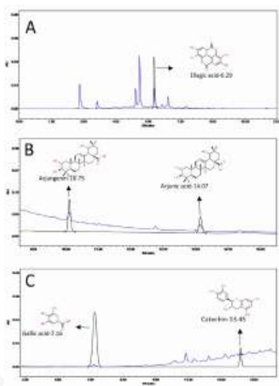
Fig. 1. HPLC-based Phytochemically analysis of TAE. The compounds in TAE were A) ellagic acid (365 nm wavelength); B) arjungenin and arjunic acid (210 nm wavelength); and C) gallic acid and catechin (270 nm wavelength). In the chromatograms, the black line represents standards for phytochemicals and the blue line represents phytochemicals identified in test samples.
