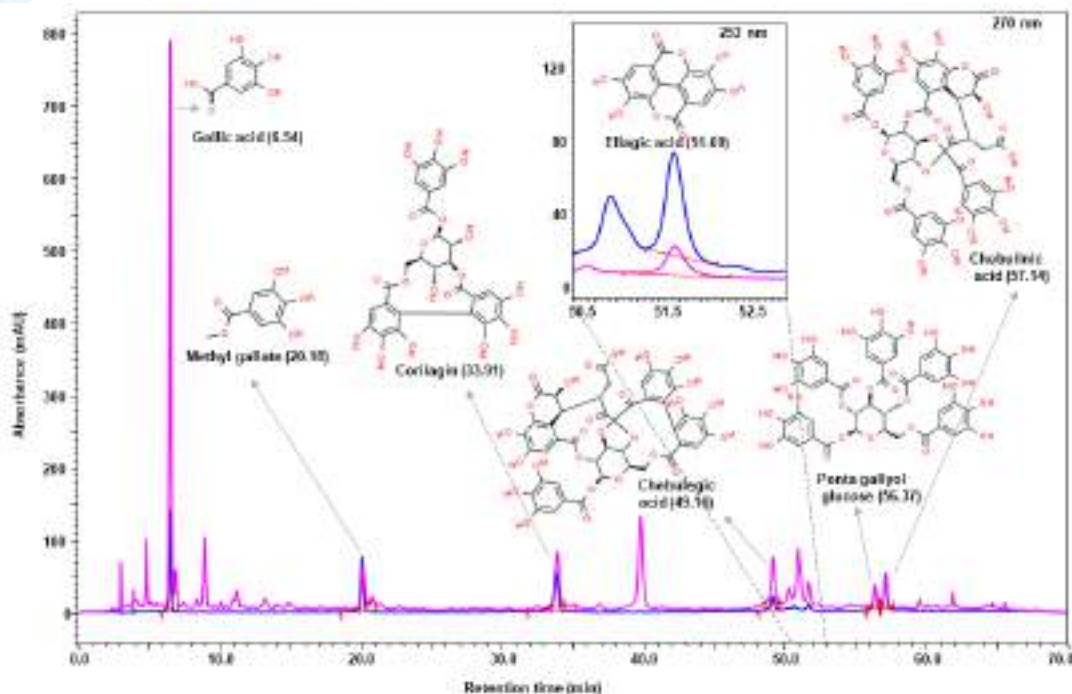
Fig. 1. Ultra High Performance Liquid Chromatography (UHPLC) equipped with Photo Diode Array (PDA) detector analysis of PhyTer tablet. In PhyTer tablet analysis, the several compounds were observed at 270 nm wavelength generally gallic acid (6.54 minutes), methyl gallate (20.18 minutes), corilagin (33.91 minutes), chebulegic acid (49.16 minutes), penta gallyol glucose (56.37 minutes), and chebulinic acid (57.14 minutes); at 253 nm wavelength ellagic acid (51.69 minutes). In the chromatograms, the blue line shows the mix standards and pink line indicates the test sample.
